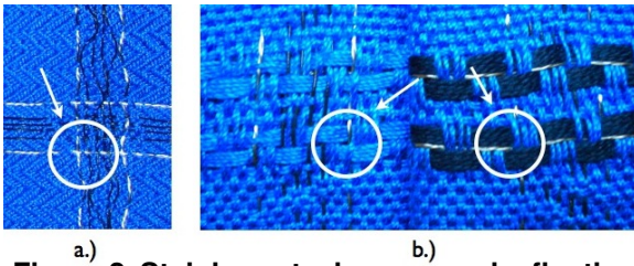
Figure 2. Stainless steel as sensor by floating wires (a) and double weave, (b)
