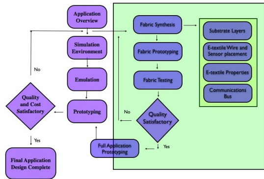
Figure 1. Expanded E-textile design flow
